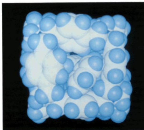
Figure 11. MM2-optimized complex of Kyuphane tetracation 10a and the linear conformation of \alpha -PNA: (a, top) stick figure; (b, bottom) head-on space-filling model demonstrating the phenyl "plug" in the hydrophobic cage face, SYBYL van der Waals radii.
