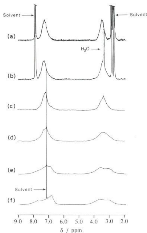
Figure 4. 1 H NMR spectra of Kyuphane at (a) 398, (b) 298, (c) 273, (d) 223, (e) 198, and (f) 173 K in the following solvents: DCON(CD 3 ) 2 , (a) and (b); CDCl 3 -CS 2 (3:7 v/v), (c)–(f).
