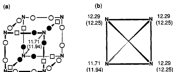
Figure 7. C_i symmetry of 1a and 10a as illustrated by (a) three different environments for the \text{CH}_2 's bonded to N and (b) the N...N diagonal distances (Å). Parenthetical values belong to 10a .
