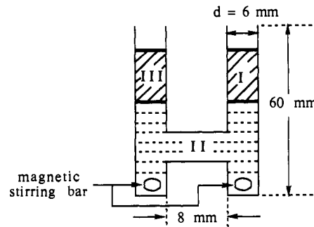
Figure 1. H-type cell used to study the transport of various organic guests.
